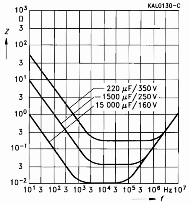
Impedance Z versus frequency f Typical behavior V_R \geq 160 Vdc
