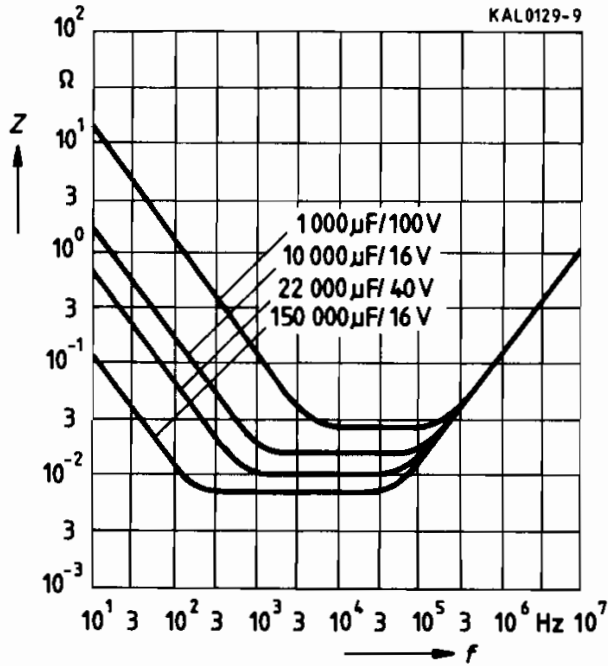
Impedance Z versus frequency f Typical behavior V_R \leq 100 Vdc
