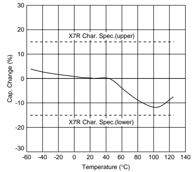
X7R Characteristics
