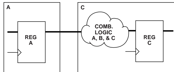
Figure 6-4 Combinatorial Logic Path Split Across Boundaries (Inefficient Use of Design Resources)
