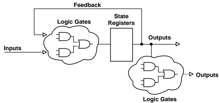
Figure 7-2 Parts of a State Machine
