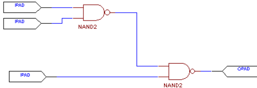
Figure 4-3 Incorrect Port Design (Without Buffers)
