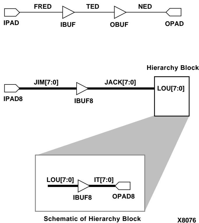
Figure B-2 Locking I/Os to Pin Locations
