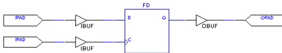
Figure 4-4 Correct Port Design (With Buffers)
