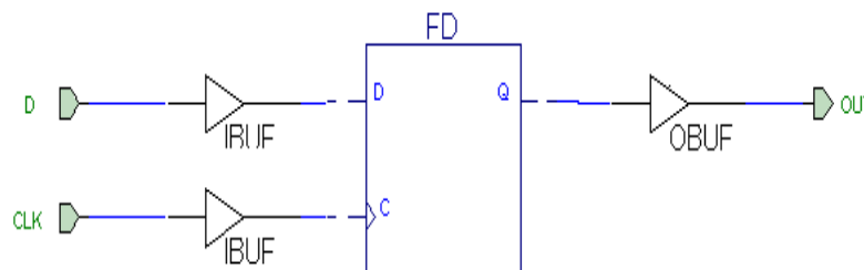
Figure 4-2 MACROS2 Schematic
