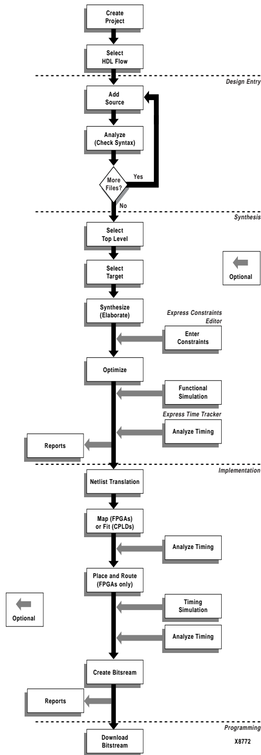
Figure 5-1 HDL Flow Project Processing
