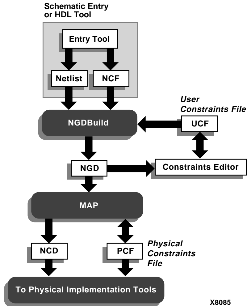
Figure B-1 Constraint Entry Flow
