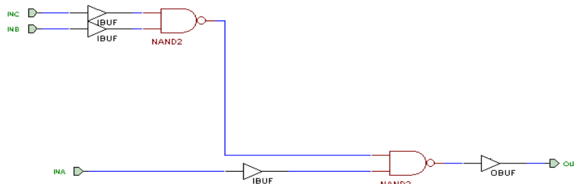
Figure 4-1 MACROS1 Schematic
