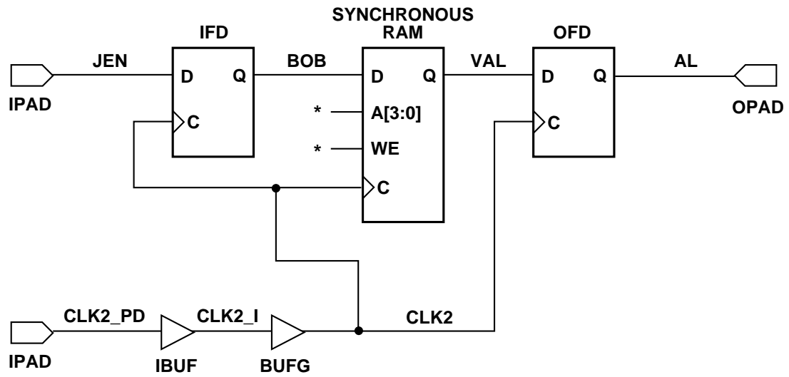
Figure B-3 Specifying Timing Constraints
