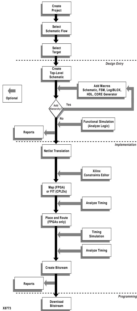
Figure 3-1 Schematic Flow Project Processing
