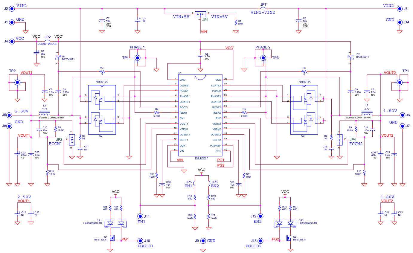
FIGURE 3. ISL6227EVAL2Z SCHEMATIC
