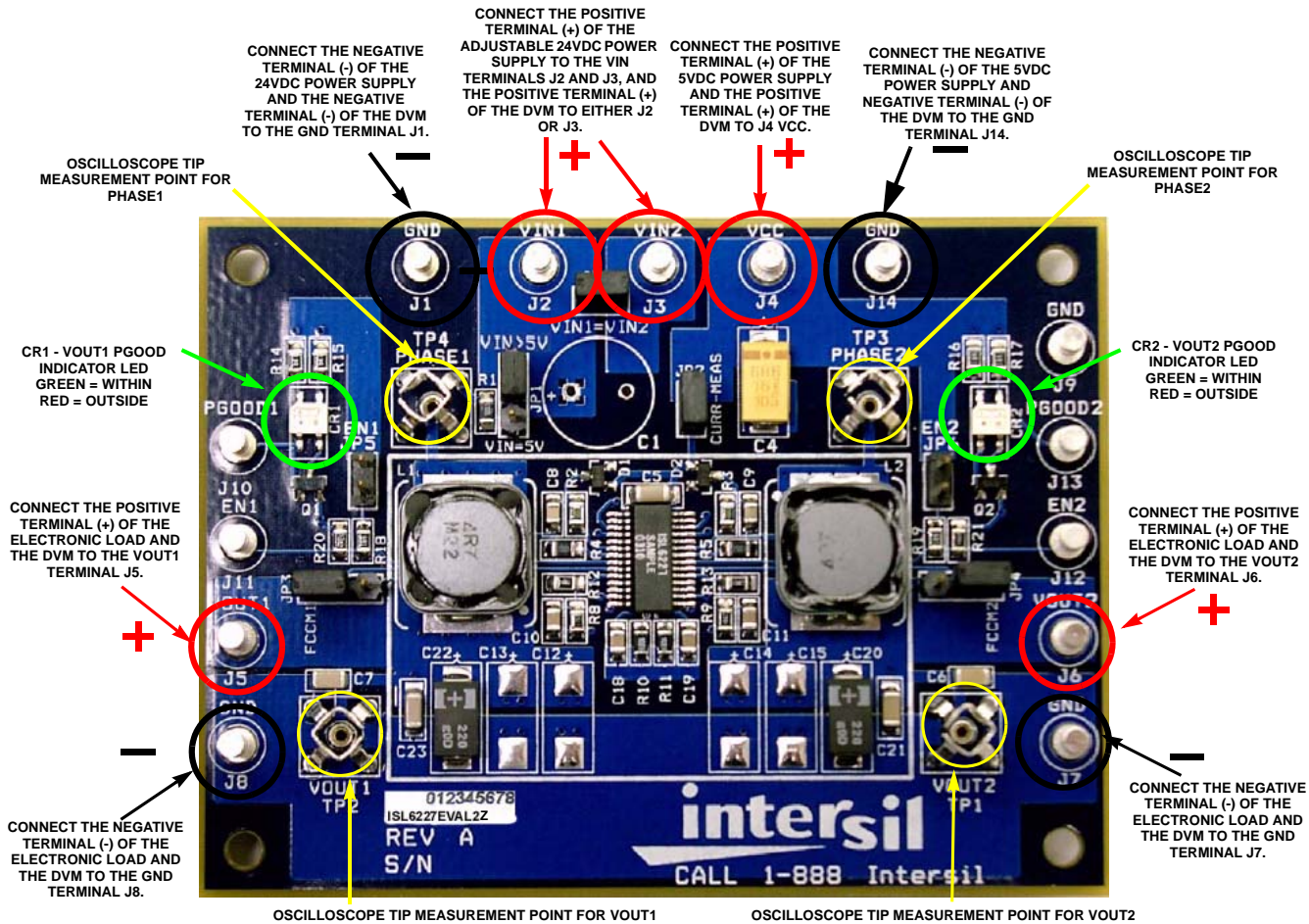
FIGURE 2. WIRING CONNECTIONS FOR ISL6227EVAL2Z
