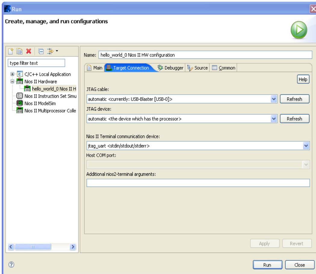
Figure 1-4. Run Dialog in the Nios II IDE
