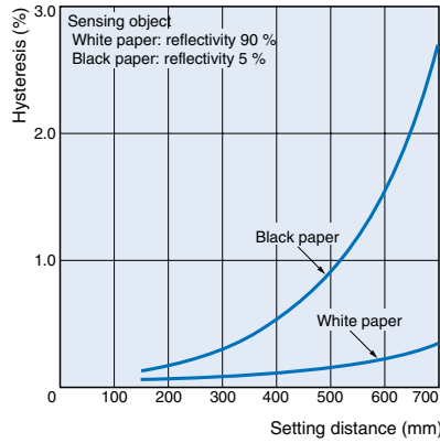
Hysteresis
