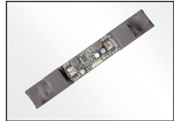
C Backlight Inverter Board (DMD42773) CAUTION: High Voltage The heat shrink tubing is used for your protection.
