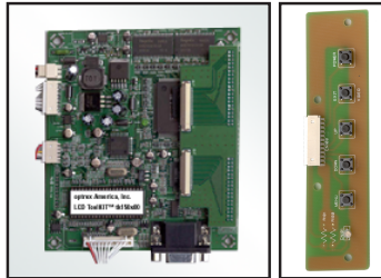
B TFT Controller Board with On-Screen Display (OSD) Board (VNS-AV-150XGATTL-00)
