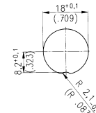
Panel Cutout
