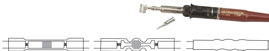
1. Strip wires 3/8" and insert into crimp barrel of the connector
