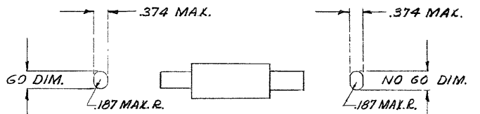
SUGGESTED PLUG GAGE DESIGN
