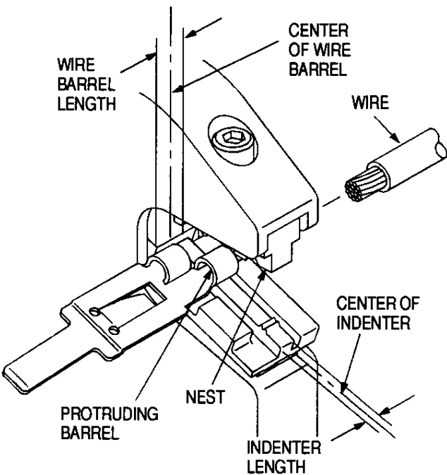
Figure 4 cad
