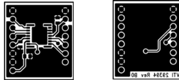
Figure 2 Layouts of SCA3000 PWB version B.
