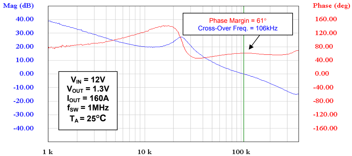
Fig. 3: Bode Plot
