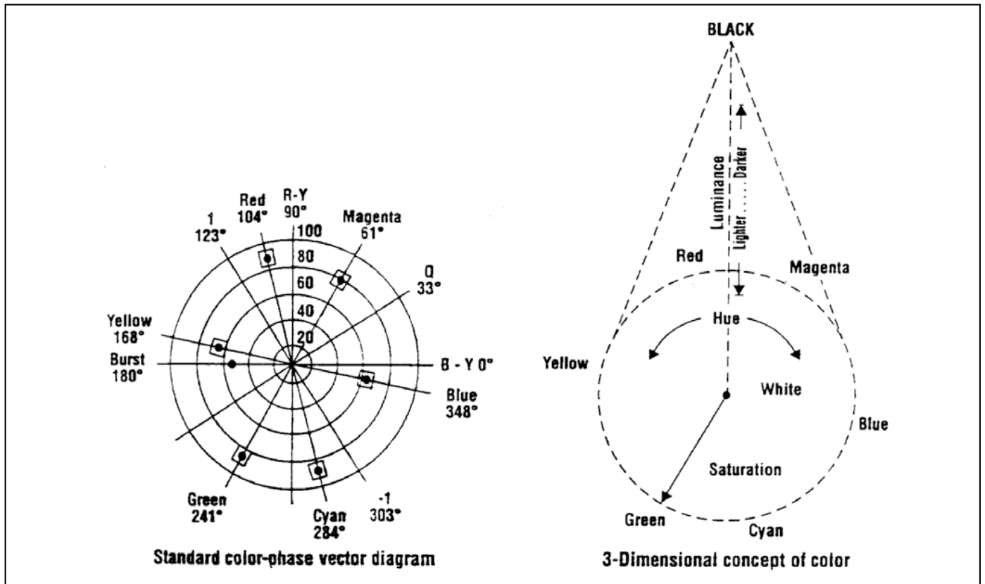
Fig. 3. Elements of Color Television Signal
