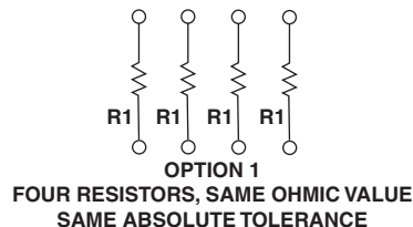
FIGURE 1 - SCHEMATICS 1)
