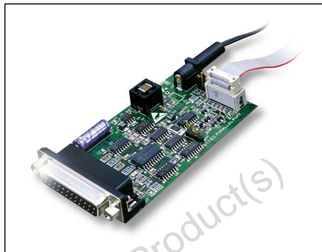
Figure 1: ST7-STICK Programmer
