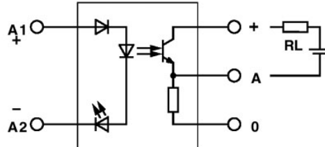
Output: 2-wire, floating, minus switching
