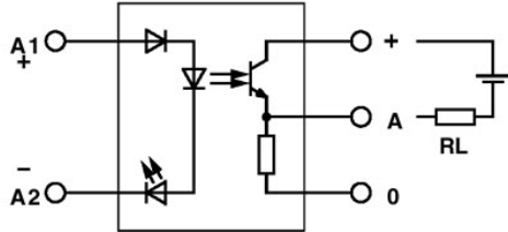
Output: 2-wire, floating, plus switching
