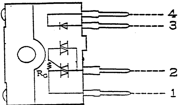
Pin Nos. and internal connection diagram
