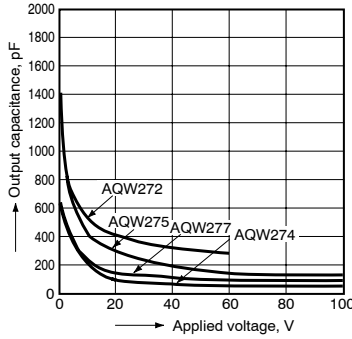
17. Applied voltage vs. output capacitance characteristics
