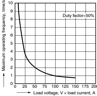
16. Maximum operating frequency vs. load voltage/current characteristics
