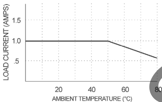
Max. Load Current vs. Temp.
