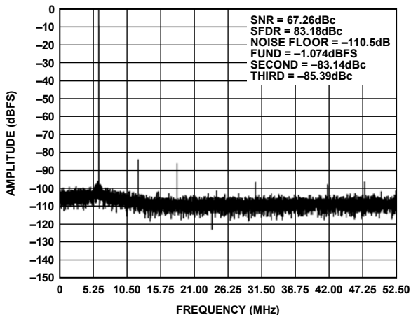
Figure 36. Single Tone Distortion AD8352 Driving AD9445, Encode Clock @ 105 MHz with f_c @ 100 MHz ( A_v = 10 dB), See Figure 34
