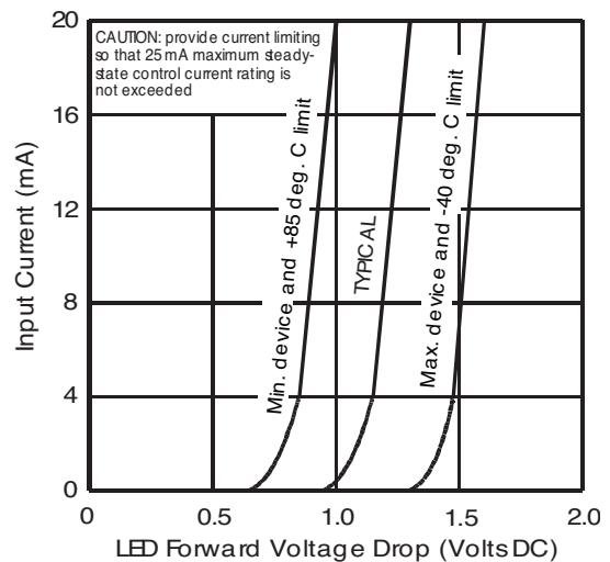
Figure 6. Input Characteristics (Current Controlled)
