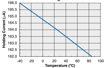
Holding Current
