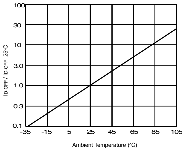
Figure 5. Typical Normalized Off-State Leakage
