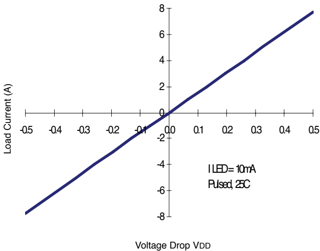
Figure 3. Typical Linearity Characteristics
