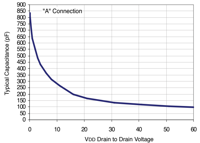
Figure 2. Typical Output Capacitance
