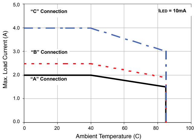
Figure 1. Current Derating Curves
