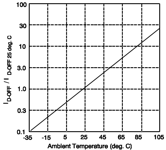
Figure 4. Typical Normalized Off-State Leakage
