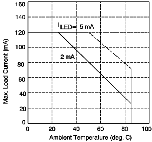
Figure 1. Typical Current Derating Curve
