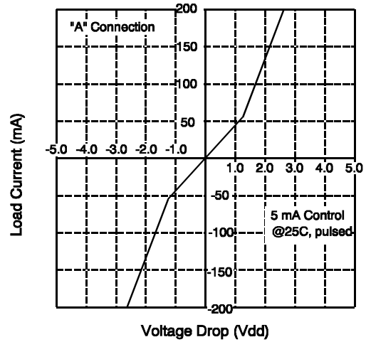
Figure 2. Linearity Characteristics
