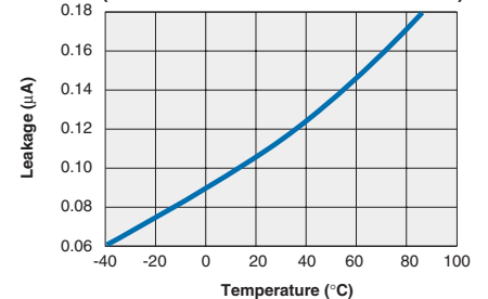
LAA125L Typical Leakage vs. Temperature (Measured across Pins 5 & 6 or 7 & 8)
