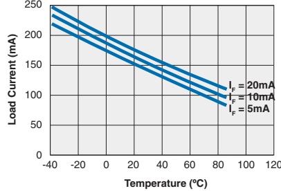
LAA125L Typical Load Current vs. Temperature
