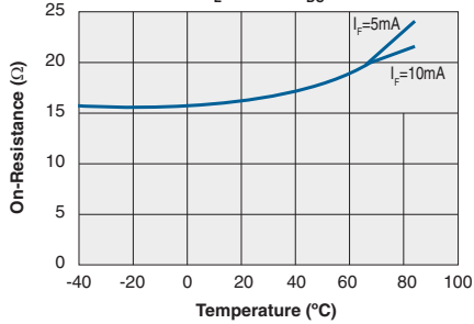
Typical On-Resistance vs. Temperature AC/DC Configuration ( I_L=150mA_{DC} )
