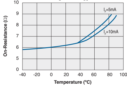
Typical On-Resistance vs. Temperature - DC Configuration ( I_L=150mA_{DC} )
