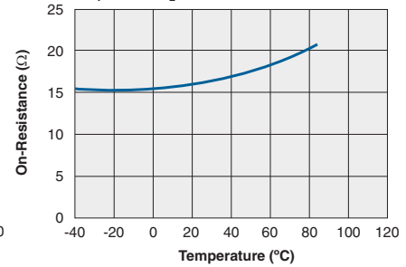
Typical On Resistance vs. Temperature ( I_F=5mA; I_L=100mA Instantaneous)
