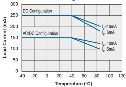
Typical Load Current vs. Temperature ( N=50, T_A=25°C )
