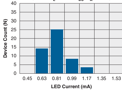
Typical I_F for Switch Dropout (N=50, I_L=170mA_{DC} , T_A=25^\circ C )
