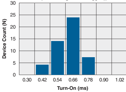
Typical Turn-On Time (N=50, I_F=5mA , I_L=170mA_{DC} , T_A=25^\circ C )
