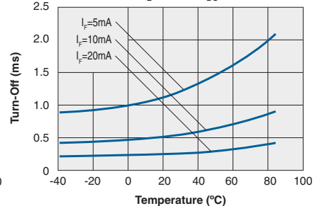
Typical Turn-Off vs. Temperature ( I_L=170mA_{DC} )
