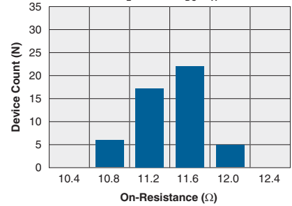
Typical On-Resistance Distribution (N=50, I_L=170mA_{DC} , T_A=25^\circ C )
