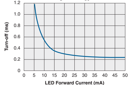
Typical Turn-Off vs. LED Forward Current ( I_L=170mA_{DC} )
