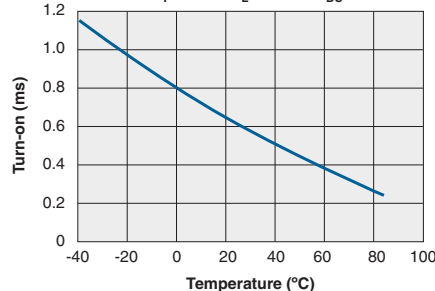
Typical Turn-On vs. Temperature ( I_F=5mA , I_L=170mA_{DC} )
