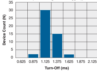
Typical Turn-Off Time (N=50, I_F=5mA , I_L=170mA_{DC} , T_A=25^\circ C )
