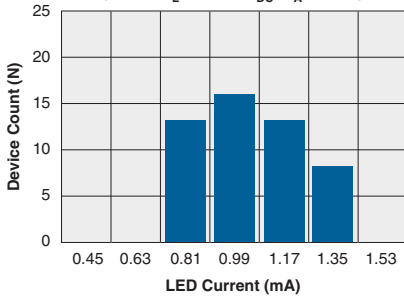
Typical I_F for Switch Operation (N=50, I_L=170mA_{DC} , T_A=25^\circ C )
