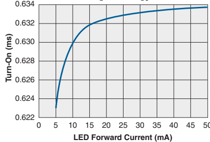
Typical Turn-On vs. LED Forward Current ( I_L=170mA_{DC} )
