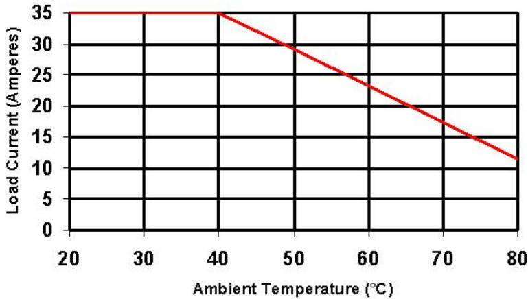
HS201DR w/50A Single SSR
