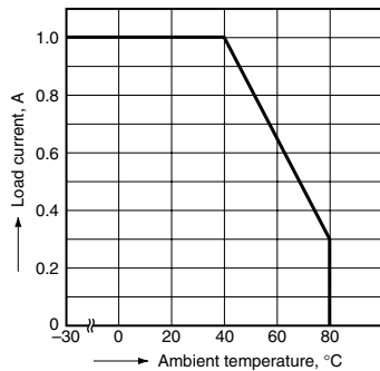
1. Load current vs. ambient temperature (AC/DC output)
