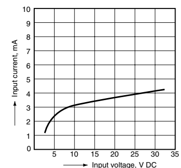
4.-(2) Input current vs. input voltage characteristics (DC input) Tested sample: AQCD3-IM4/24 V DC
