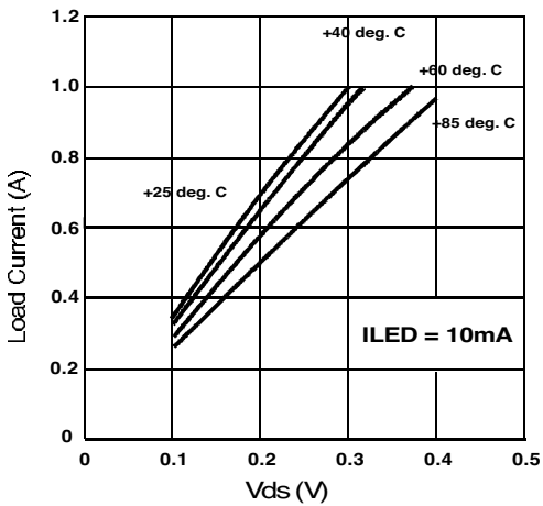
Figure 3. Typical On-Characteristics
