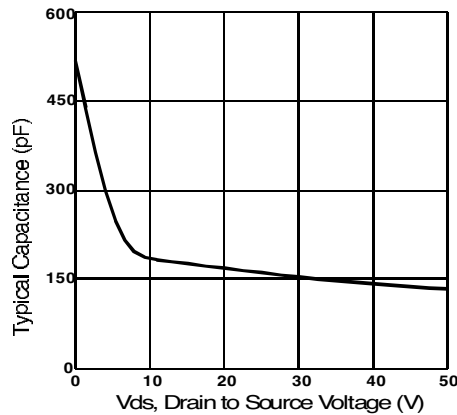
Figure 9. Typical Output Capacitance
