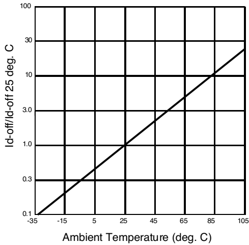
Figure 5. Typical Normalized Off-State Leakage
