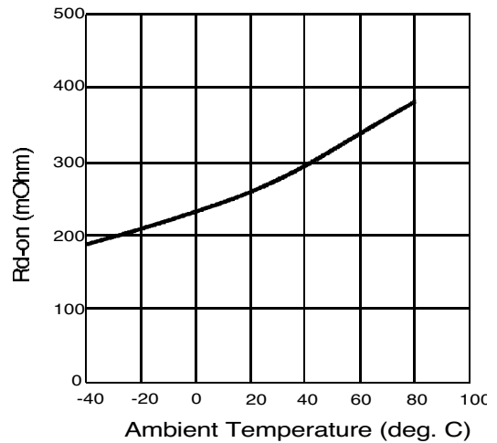
Figure 4. Typical On-Resistance
