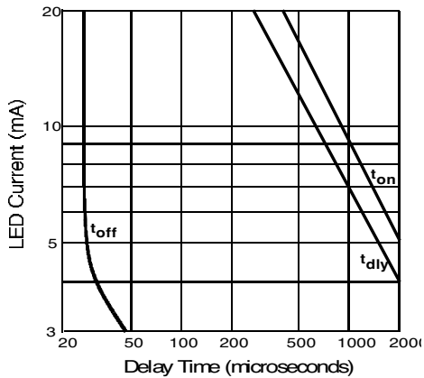
Figure 7. Typical Delay Times
