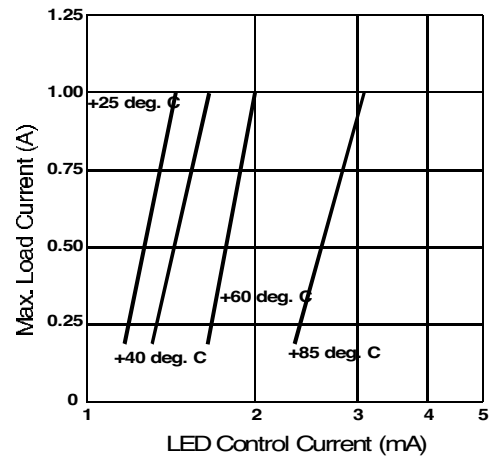
Figure 2. Typical Control Current Requirements
