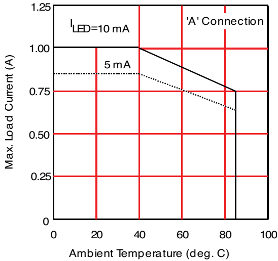
Figure 1. Current Derating Curves*
