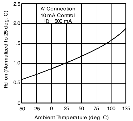
Figure 4. Typical Normalized On-Resistance
