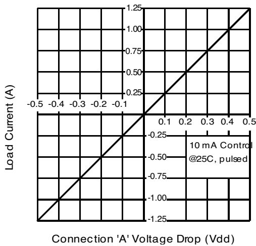
Figure 3. Linearity Characteristics
