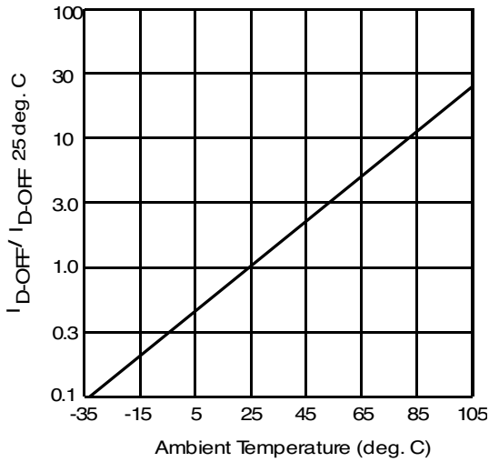
Figure 5. Typical Normalized Off-State Leakage
