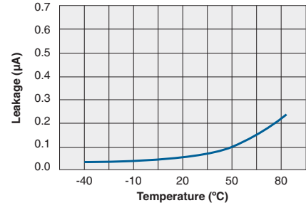
Typical Leakage vs. Temperature (V L =800V p )
