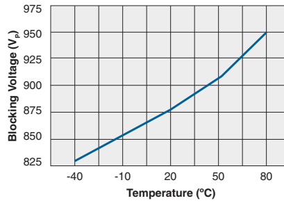
Typical Blocking Voltage vs. Temperature
