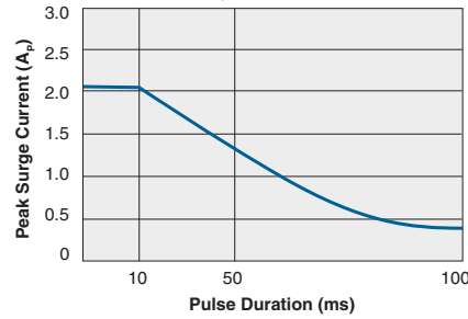
Maximum Surge Current (Non-Repetitive) (T J =50°C max)
