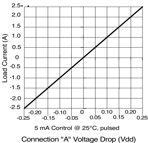
Figure 3. Linearity Characteristics
