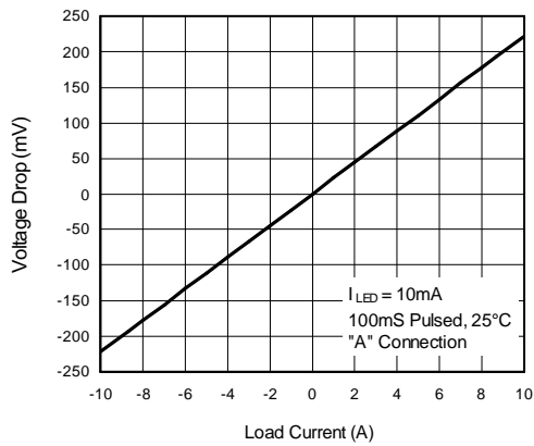
Figure 3. Linearity Characteristics
