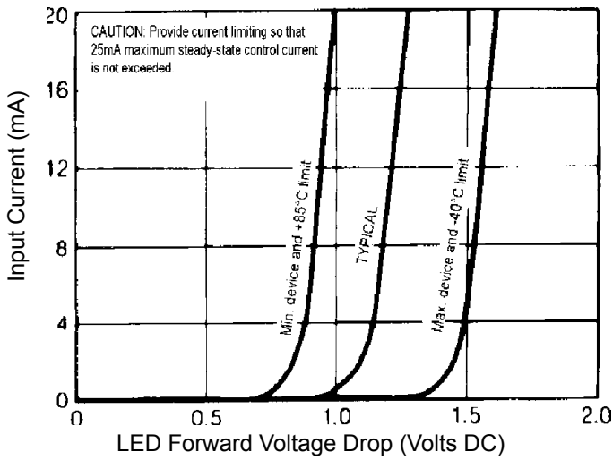
Figure 5. Input Characteristics (Current Controlled)
