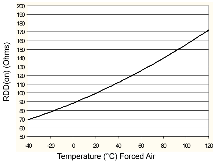
Figure 3. Typical On-Resistance
