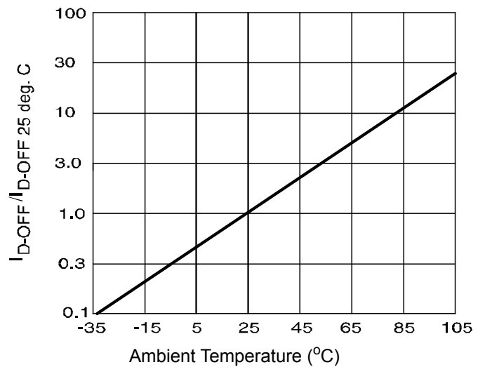
Figure 4. Typical Normalized Off-State Leakage
