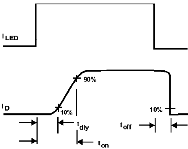
Figure 7. Delay Time Definitions
