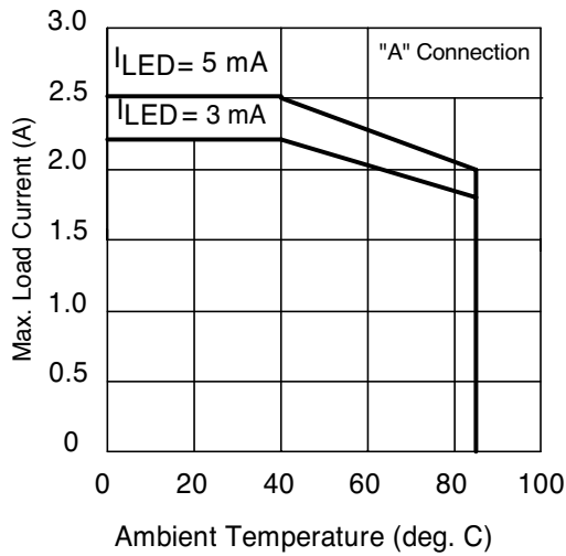
Figure 1. Current Derating Curves*
