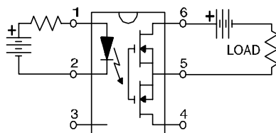
"B" Connection
