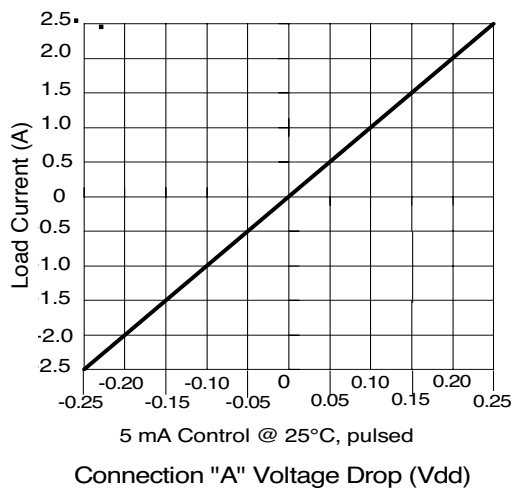
Figure 3. Linearity Characteristics
