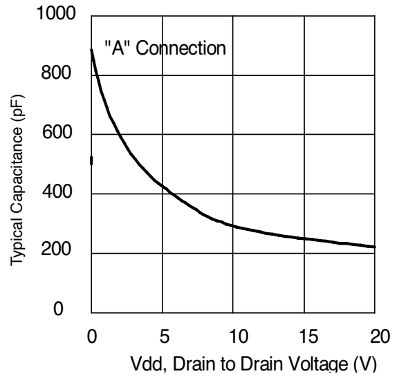
Figure 2. Typical Output Capacitance
