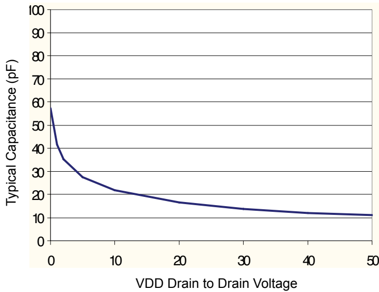
Figure 9. Typical Output Capacitance
