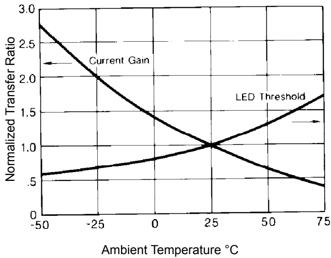
Figure 9. Typical Control Threshold and Transfer Ratio
