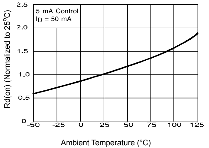
Figure 4. Typical On-Resistance
