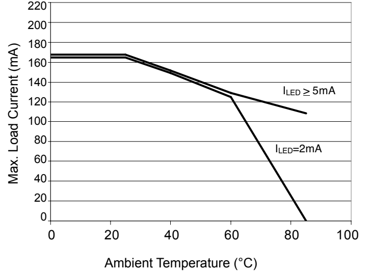
Figure 2. Current Derating Curves (PVA3354N, PVA2352N)
