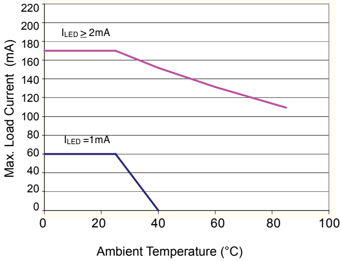
Figure 1. Current Derating Curves (PVA3324N)
