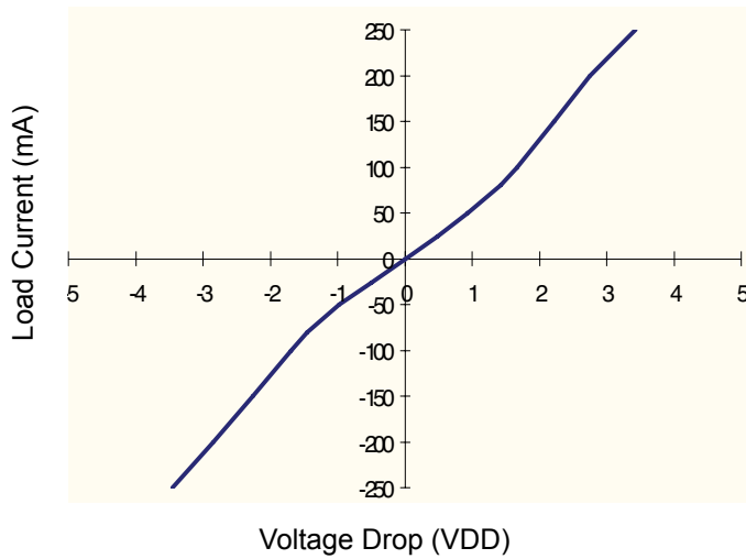
Figure 3. Typical On Characteristics
