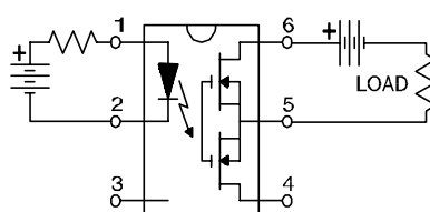
"B" Connection
