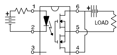
"C" Connection
