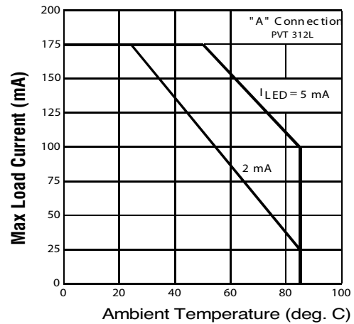
Figure 2. Typical Current Derating Curves
