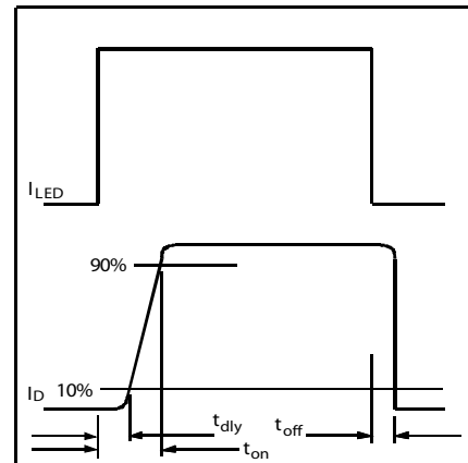
Figure 8. Delay Time Definitions
