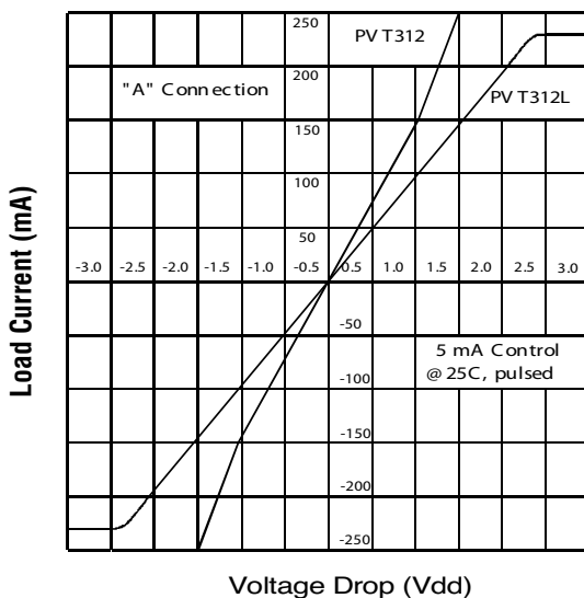
Figure 3. Linearity Characteristics
