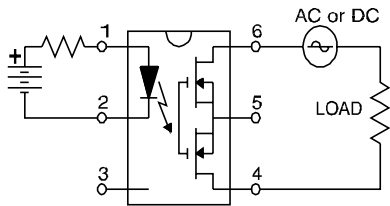
"A" Connection
