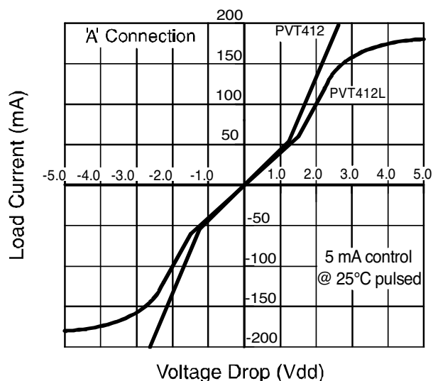
Figure 3. Linearity Characteristics
