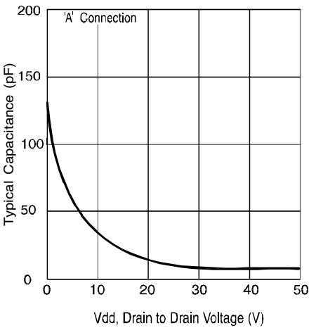
Figure 9. Typical Output Capacitance
