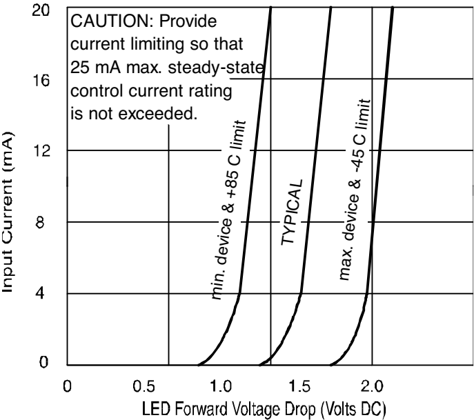
Figure 6. Input Characteristics (Current Controlled)
