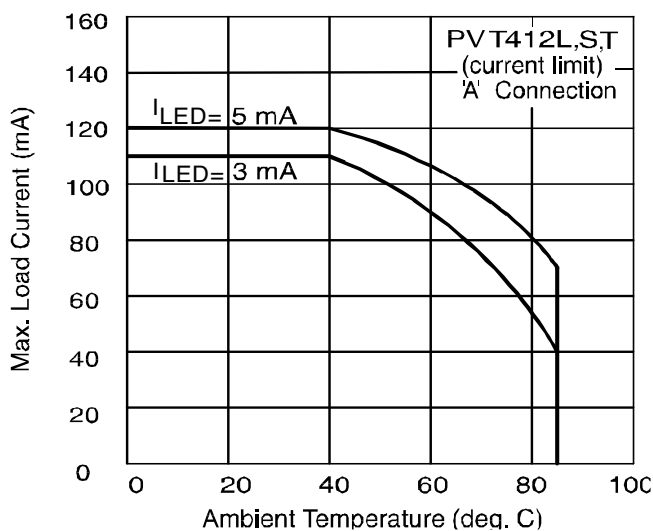
Figure 2. Current Derating Curves*
