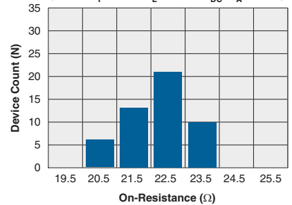
Form-A Typical On-Resistance Distribution (N=50, I_F=5\text{mA} , I_L=120\text{mA}_{DC} , T_A=25^\circ\text{C} )
