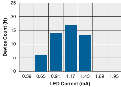
Form-A Typical I_F for Switch Dropout (N=50, I_L=120\text{mA}_{DC} , T_A=25^\circ\text{C} )
