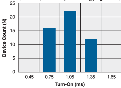
Form-A Typical Turn-On Time (N=50, I_F=5\text{mA} , I_L=120\text{mA}_{DC} , T_A=25^\circ\text{C} )
