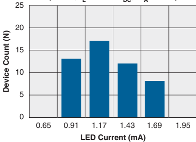
Form-A Typical I_F for Switch Operation (N=50, I_L=120\text{mA}_{DC} , T_A=25^\circ\text{C} )
