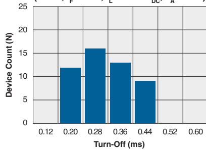
Form-A Typical Turn-Off Time (N=50, I_F=5\text{mA} , I_L=120\text{mA}_{DC} , T_A=25^\circ\text{C} )
