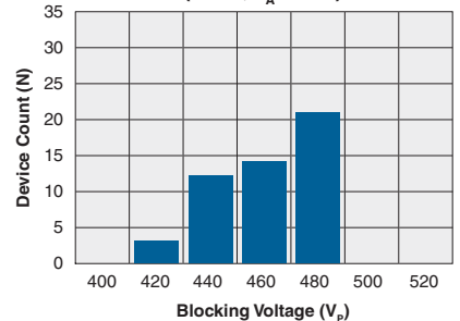
Form-A Typical Blocking Voltage Distribution (N=50, T_A=25^\circ\text{C} )
