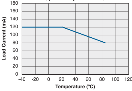
Typical Load Current vs. Temperature ( I_F=0mA, I_L=AC Peak )
