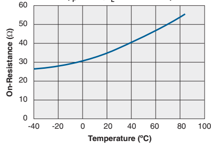
Typical On-Resistance vs. Temperature ( I_F=0\text{mA} , I_L=\text{Max Rated} )
