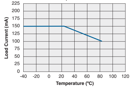
Typical Load Current vs. Temperature ( I_F=0mA )
