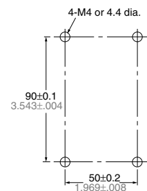
Mounting dimensions (Bottom view)
