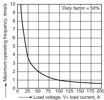
17. Maximum operating frequency vs. load voltage/current characteristics
