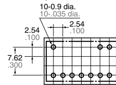
2 coil latching
