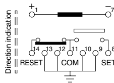
(Reset condition)
