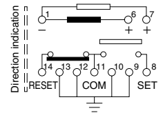
(Reset condition)
