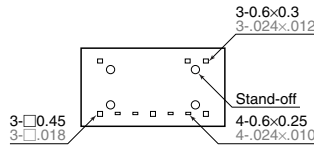
2 coil latching
