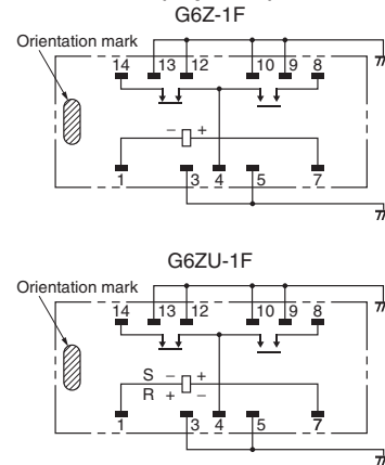
Terminal Arrangement/Internal Connections (Top View)
